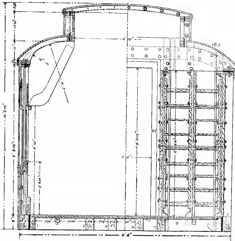
Fig. 527. Half Cross Section and Half End Elevation.
